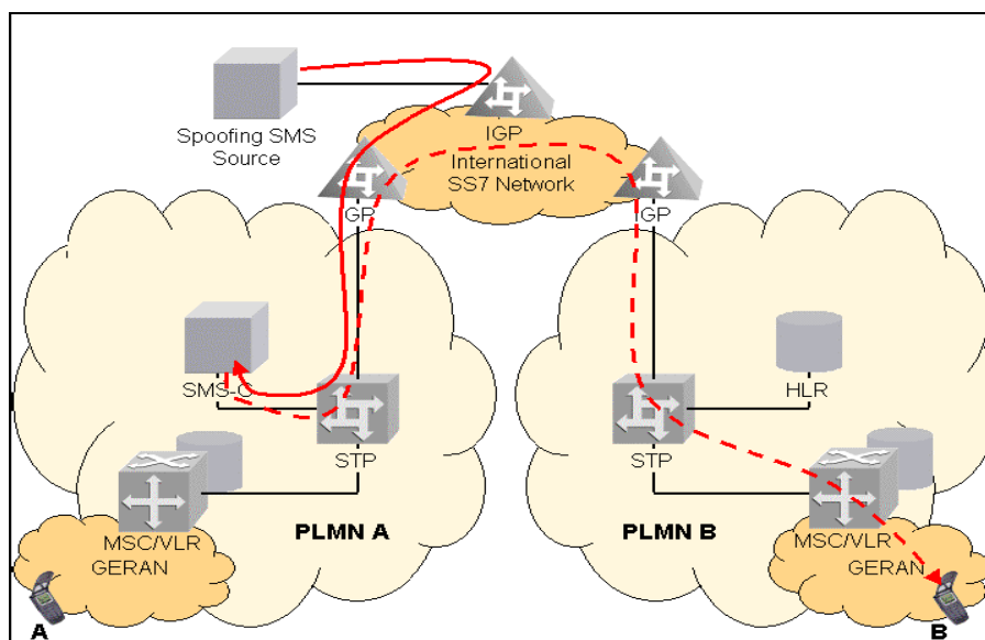
Gambar 5. SMS Spoofing Case
