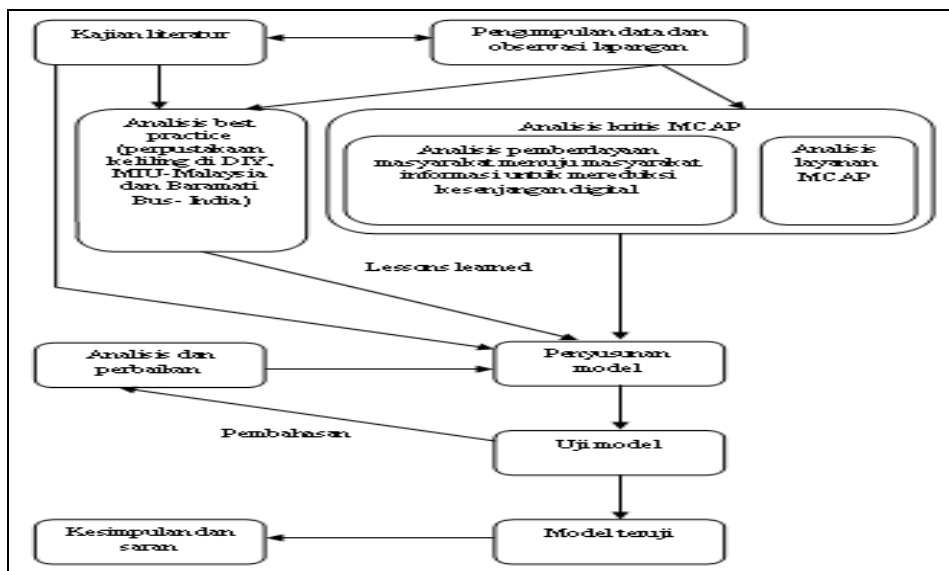
Gambar 1. Metode penelitian
