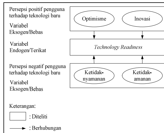
Gambar 2. Model penelitian
