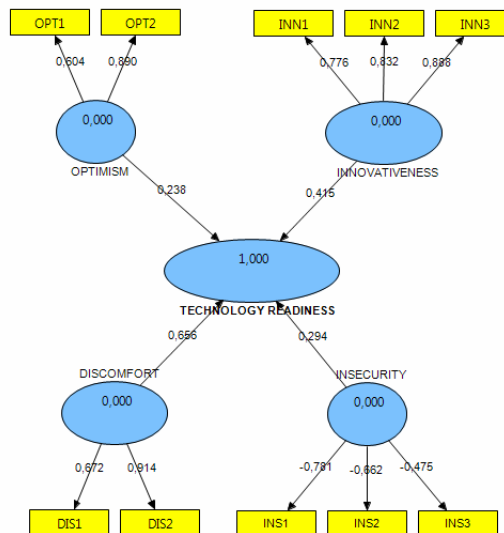
Gambar 3. Path diagram
