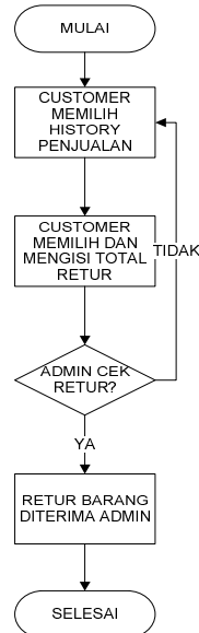
Gambar 4. Flowchart Retur Barang Customer
