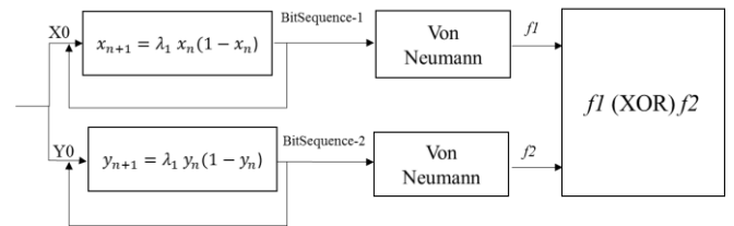
Gambar 2. Diagram blok skema chaotic random bit generator [10]
