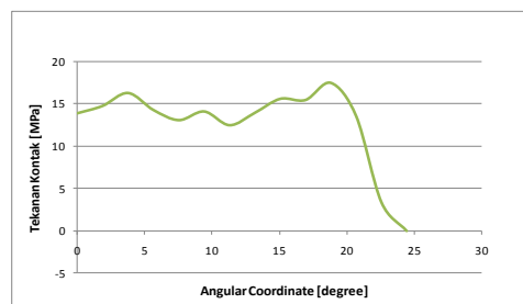
Gambar 5. Distribusi tekanan kontak CoCr-on-ST
