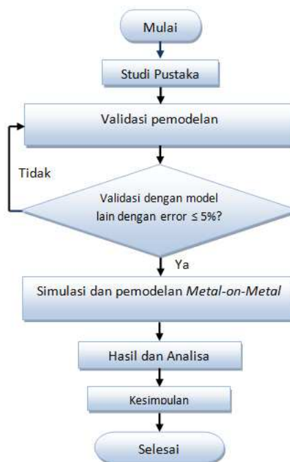
Gambar 1. Flowchart penelitian.
