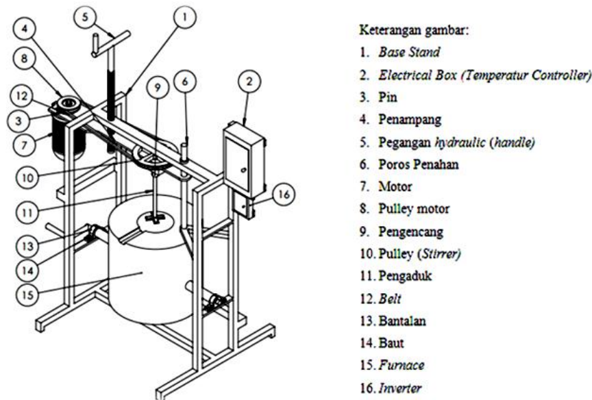
Gambar 1. Tungku stir casting
