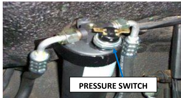
Gambar 4. Sensor pengukur tekanan refrigerant
