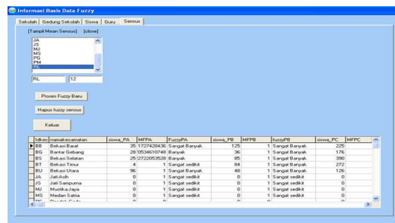
Gambar 4.4 Menu Proses & Informasi Basis Data Fuzzy
