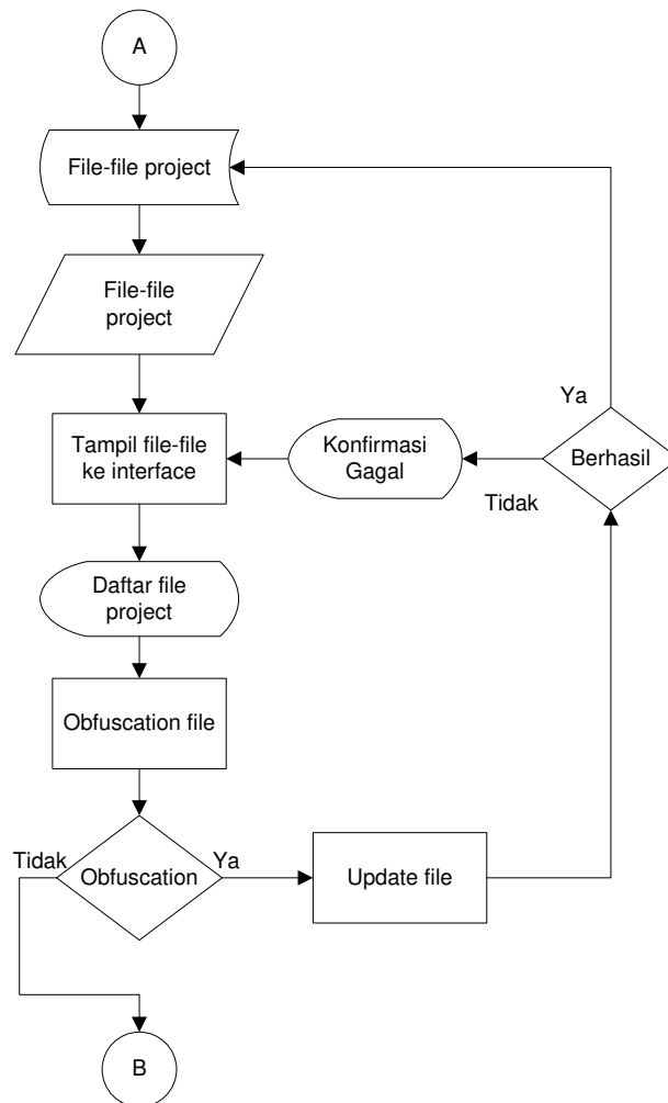
Gambar 3.1 Sistem obfuscation
