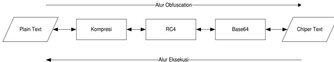
Gambar 3.2 Alur Obfuscation
