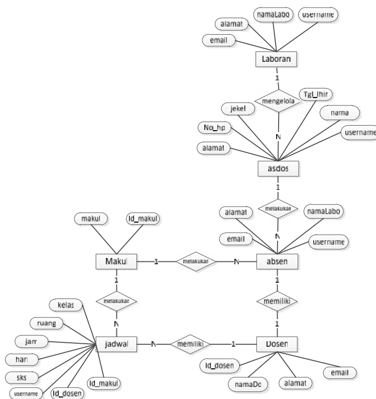
Gambar 3: Entity relation diagram
