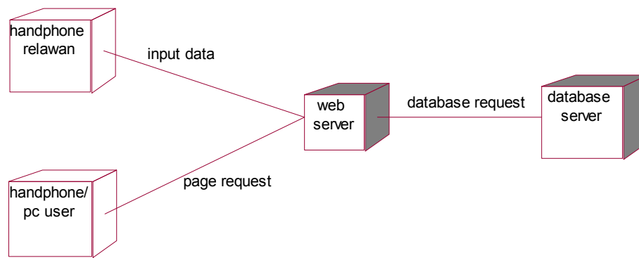
Gambar 5. Deployment diagram
