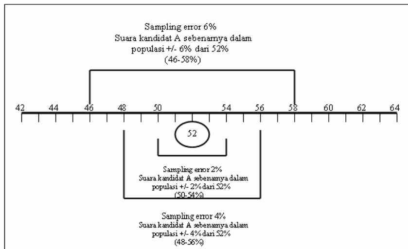
Gambar 1. Sampling error
