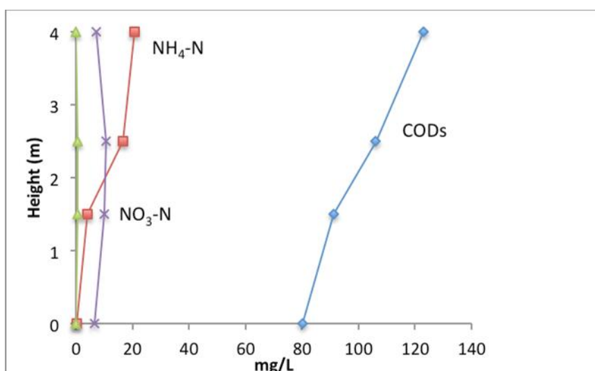
Figure 2. Profiles along the G3-DHS bioreactor height
