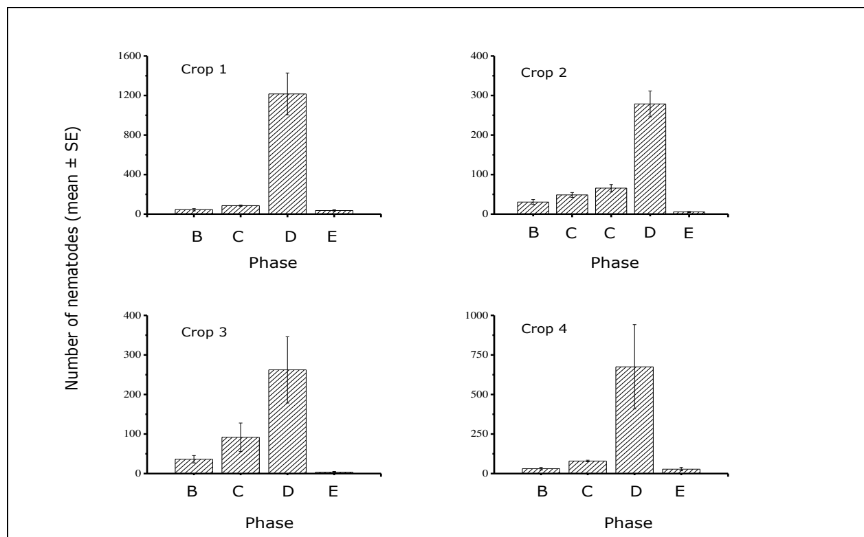
Figure 1. Number of nematode per fig during the development of F. racemosa figs. Numbers were obtained from extraction of whole figs (note the varying scale of the Y-axis).
