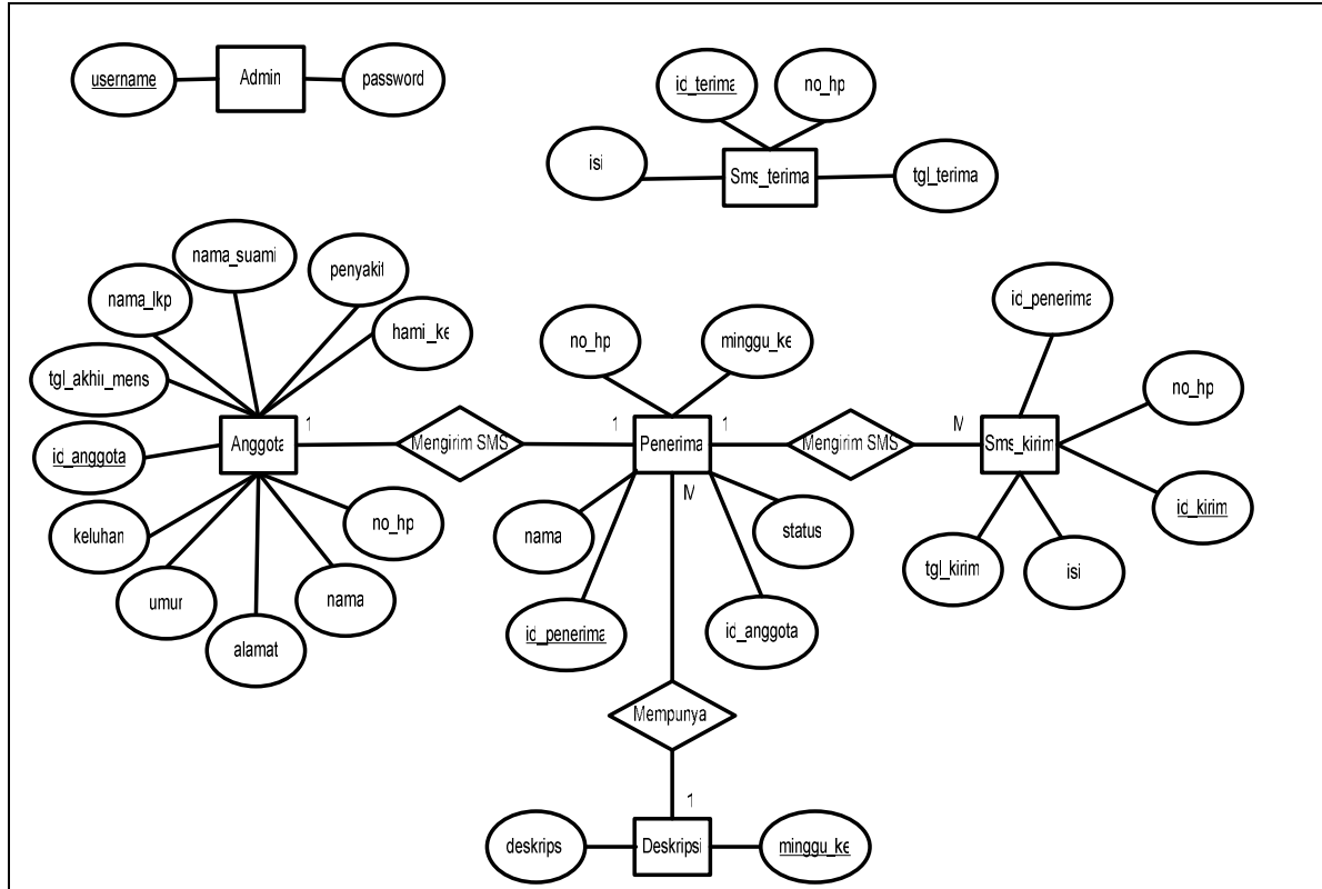
Gambar 3.7 Entity-Relationship Diagram
