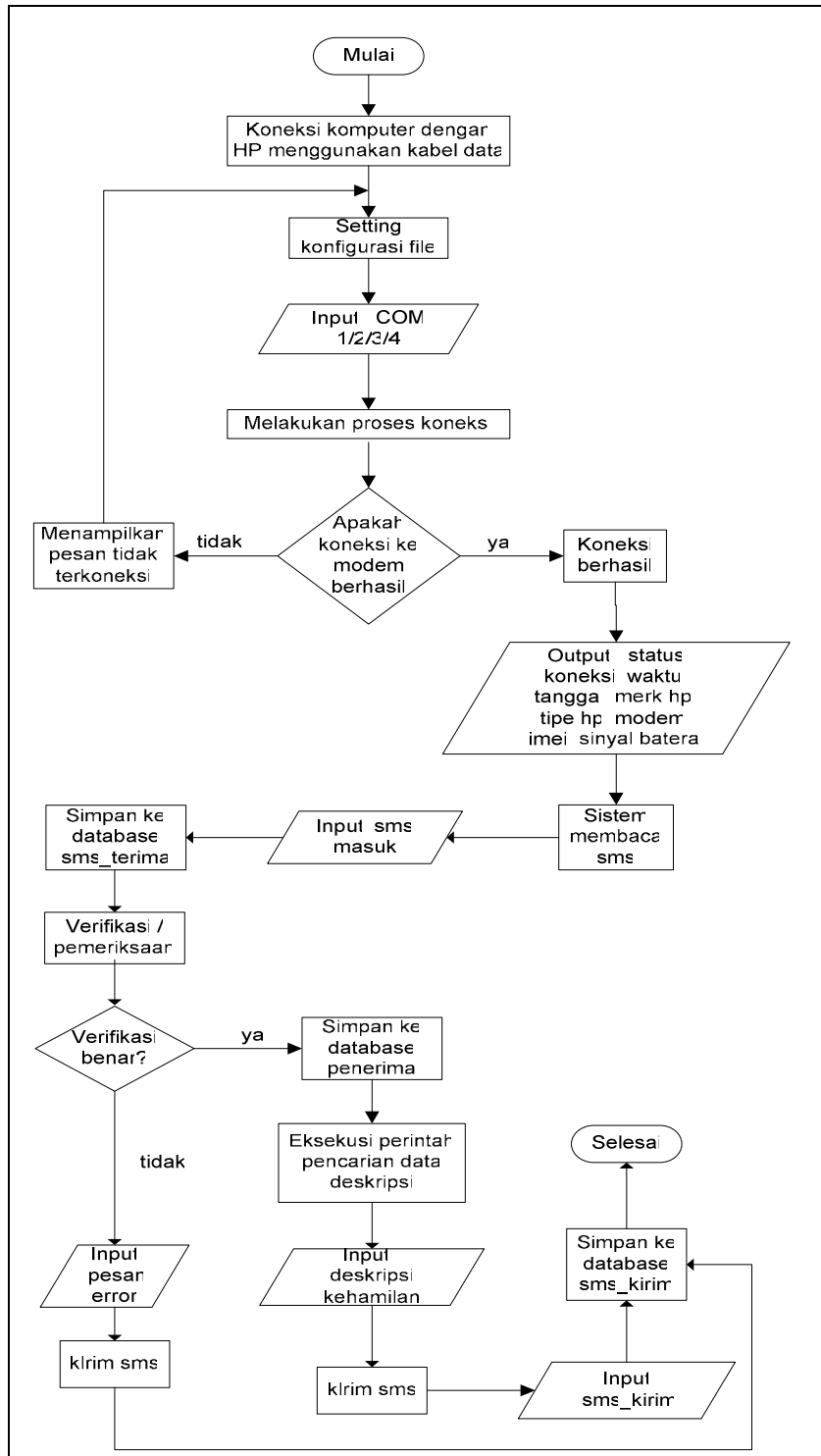
Gambar 3.6 PSPEC SMS
