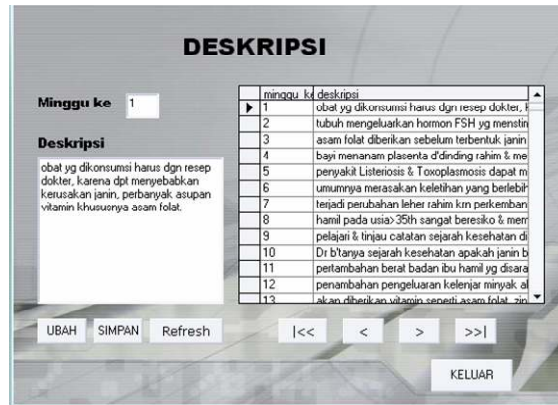
Gambar 4.4 Halaman deskripsi
