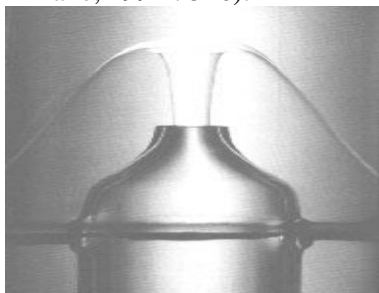
Gambar 3. Fenomena Super Fluida
