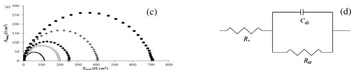
Figure 1. EIS diagrams for MS in 1.0 M HCl in the absence and presence of different concentrations of extracts of (a) Uncaria gambir (b) Tinospora cripisa and (c) Rhizophora apiculata . Concentrations: — 1.0 M HCl; ○—○ 50 ppm; ●—● 100 ppm; +++ 500 ppm and ■—■ 1000 ppm. (d) Randle circuit diagram of corrosion mechanism.
