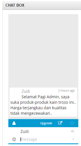
Gambar 7 Tampilan Chatbox
