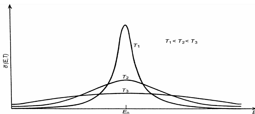
Gambar 2. Efek Doppler
