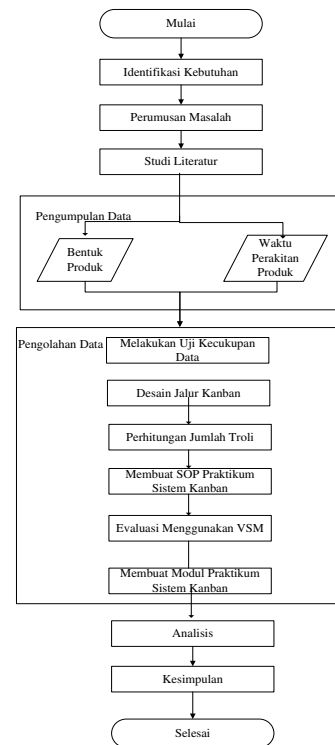
Gambar 2 Flowchart penelitian
