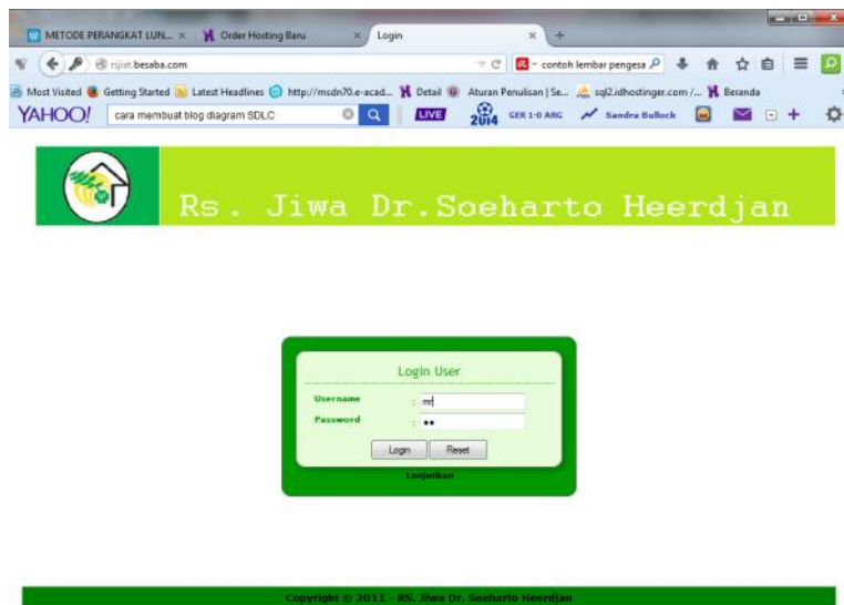
Gambar 5. Form Login
