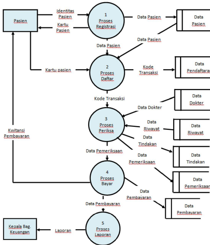
Gambar 3. DFD Level 0
