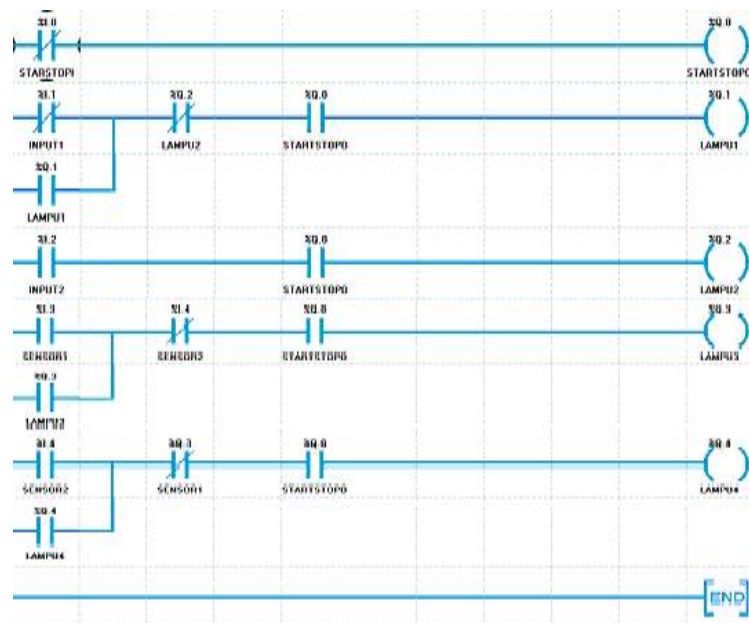
Gambar 5. Program Ladder Hydroponic.Ldr
