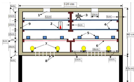
Figure 1. Incubator looks ahead
