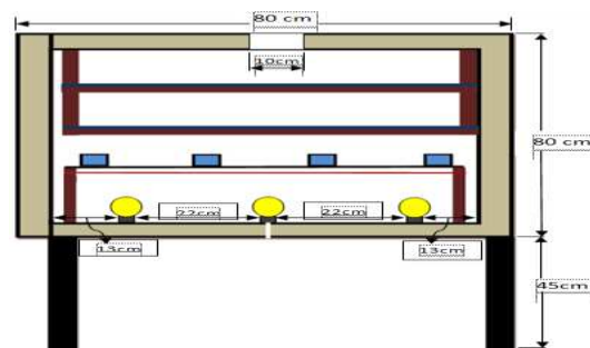
Figure 2. Incubator side view
