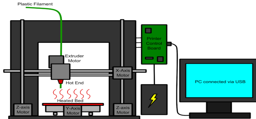
Gambar 1. Draft rancangan mesin printer 3D.
