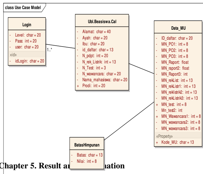
Image 3.10 Class Diagram of Scholarship SPK
