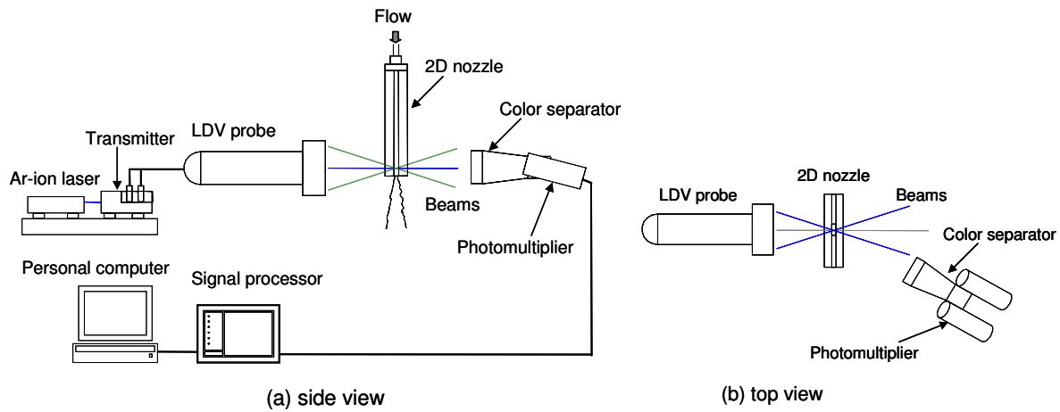
Fig. 3 Experimental setup for LDV measurement.
