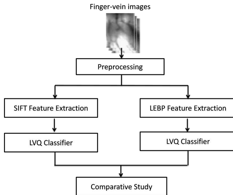
Figure. 1. Flowchart of finger-vein recognition system
