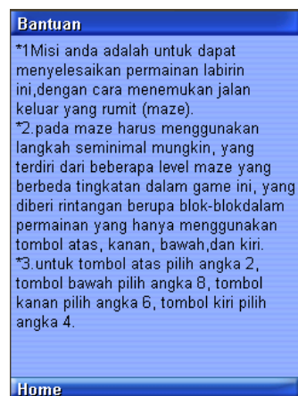
Gambar 4. Tampilan Bantuan
