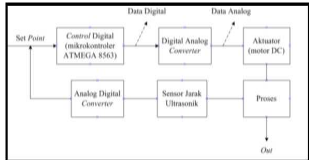
Gambar 4. Diagram blok
