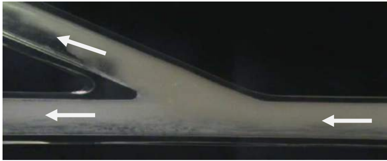
Figure 12. The current of Homogen kerosene-water to J_{mix} = 0,43 m/s
