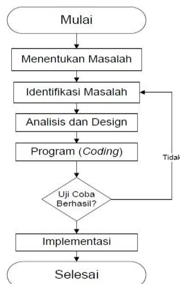
Gambar 1. Alur Penelitian
