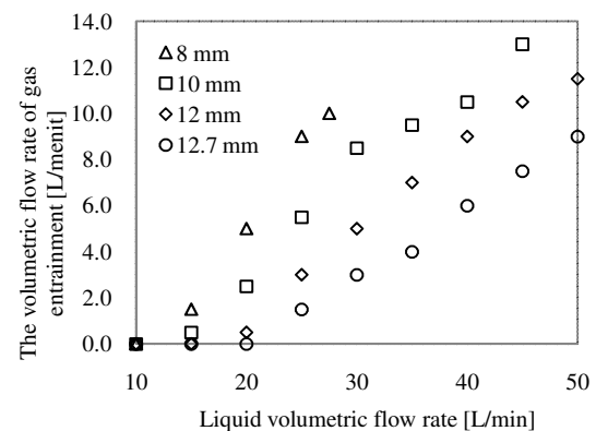
Fig. 2. Effect of liquid volumetric flow rate toward any size of nozzle diameter
