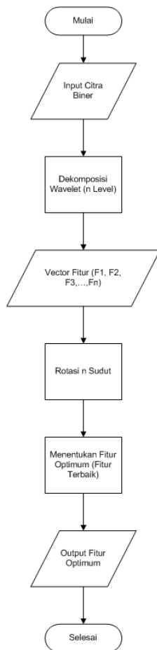
Figure 4. Feature extraction flowchart.
