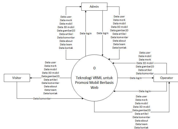
Gambar 1. DFD level 0
