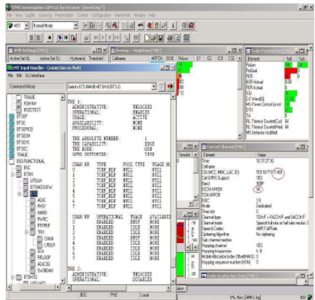
Gambar 3 Data TEMS SQI Call AMR Fullrate
