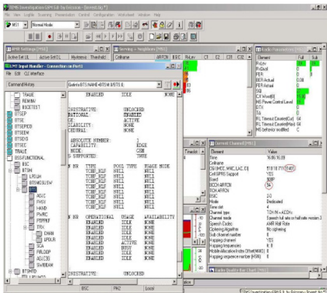
Gambar 5 Data TEMS SQT Call AMR Halfrate
