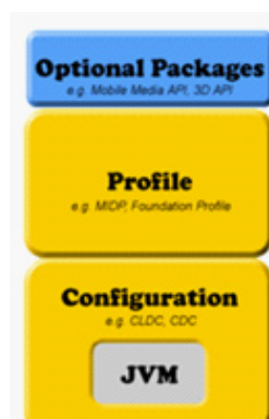
Fig. 1: J2ME Stack
