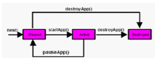
Fig. 2: MIDlet process in Java Application Manager (JAM)
