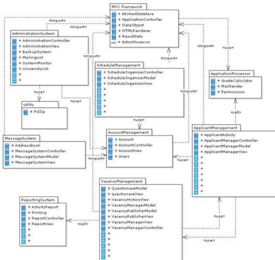
Gambar 3 Package Component
