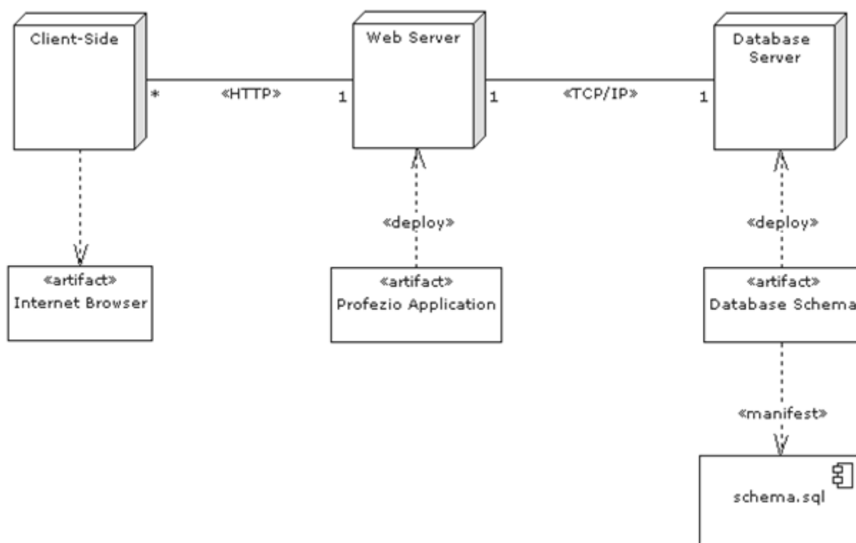
Gambar 4 Deployment Diagram
