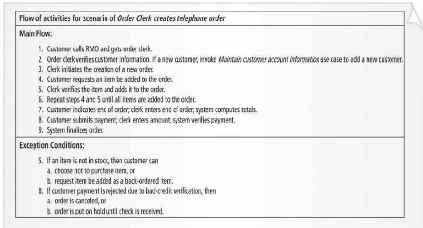
Gambar 5 Use case description (Satzinger, et al., 2005)
