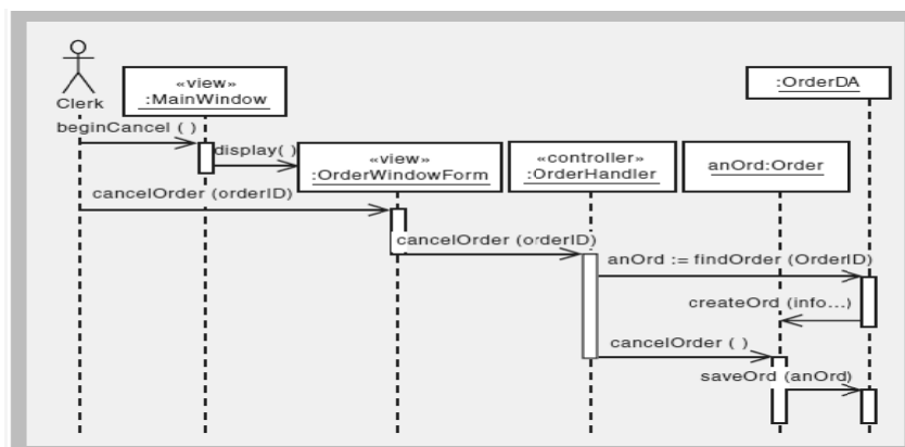
Gambar 10 View layer diagram (Satzinger, et al., 2005)
