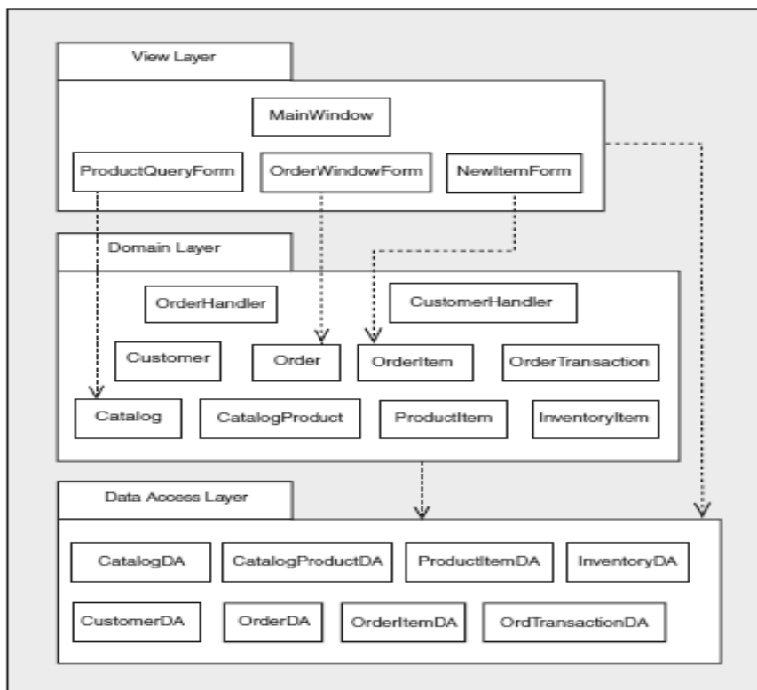
Gambar 14 Package diagram (Satzinger, et al., 2005)
