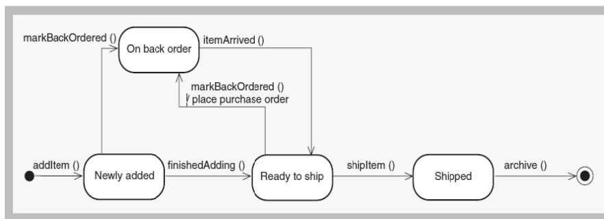
Gambar 6 State Chart (Satzinger, et al., 2005)
