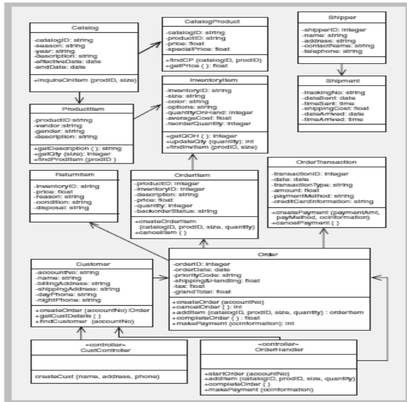
Gambar 13 Update design class diagram (Satzinger, et al., 2005)
