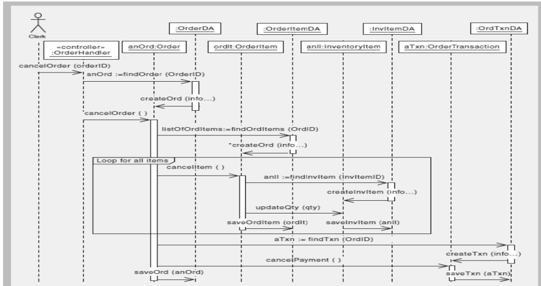
Gambar 11 Data access layer diagram (Satzinger, et al., 2005)
