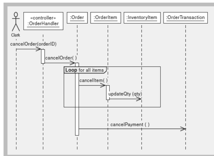
Gambar 9 First cut sequence diagram (Satzinger, et al., 2005)
