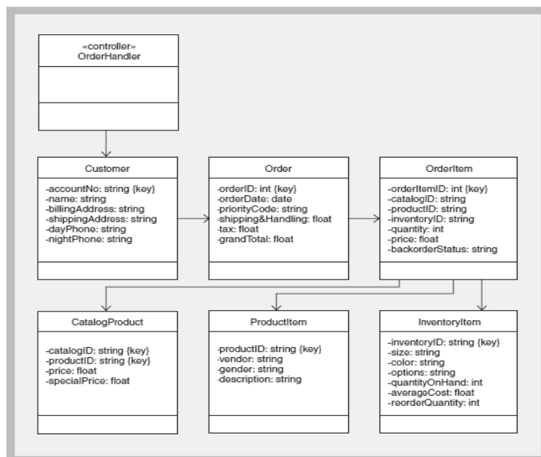
Gambar 7 First cut design class diagram (Satzinger, et al., 2005)
