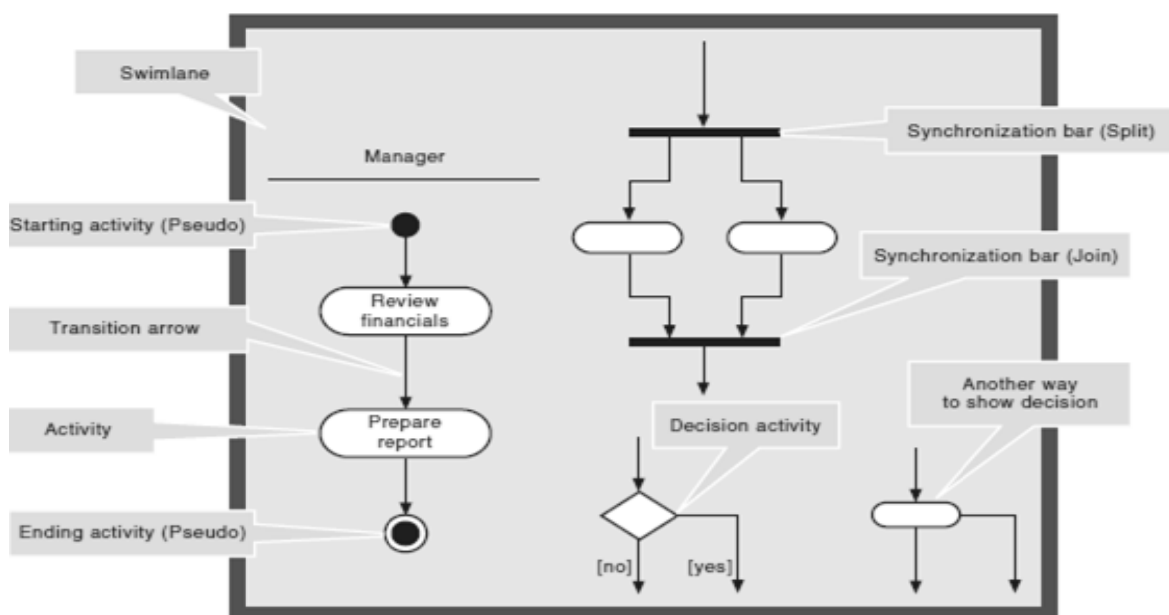
Gambar 1 Activity diagram (Satzinger, et al., 2005)
