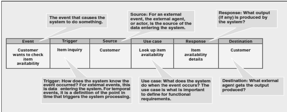
Gambar 2 Event table (Satzinger, et al., 2005)
