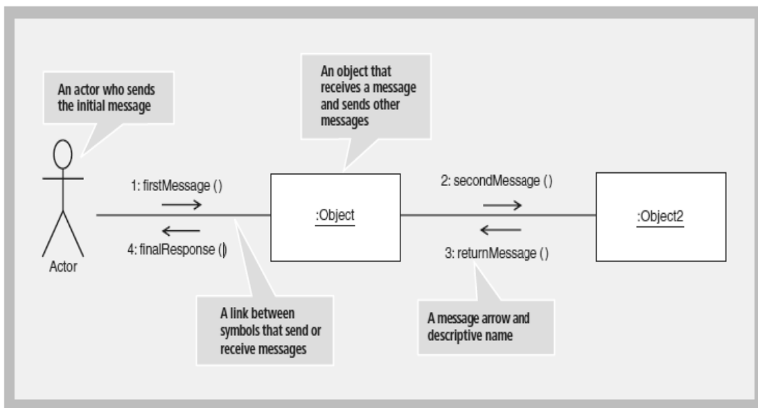
Gambar 12 Communication diagram (Satzinger, et al., 2005)
