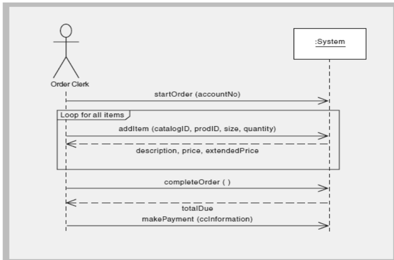
Gambar 8 Simple Sequence Diagram (Satzinger, et al., 2005).
