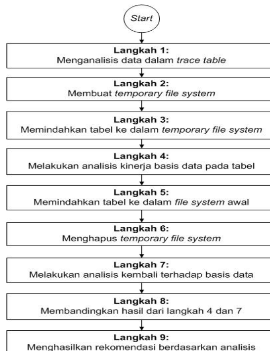
Gambar 3. Flowchart proses analisis
