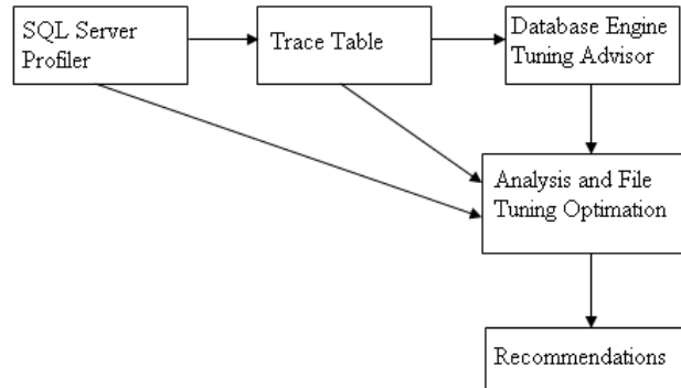
Gambar 2 Arsitektur aplikasi Analysis and File Tuning Optimization
