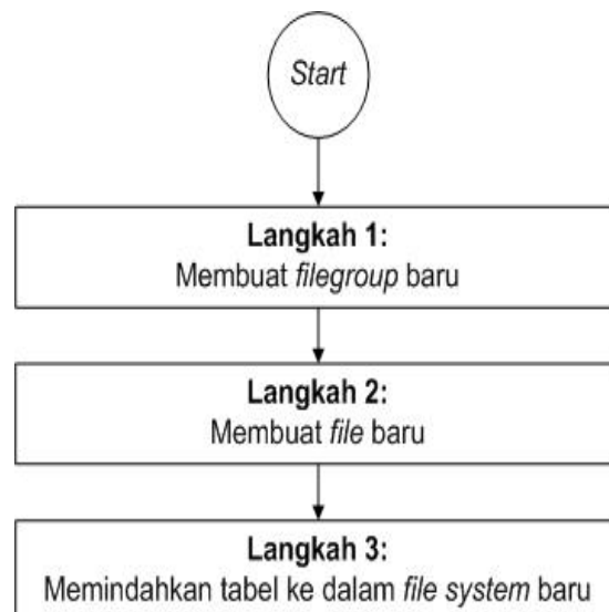
Gambar 4 Flowchart proses tuning
