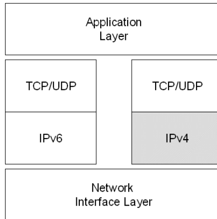
Gambar 4 Dual Stack (Rafiudin, 2005)
