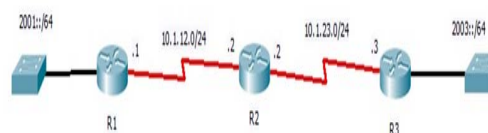
Gambar 7 Topology Jaringan
