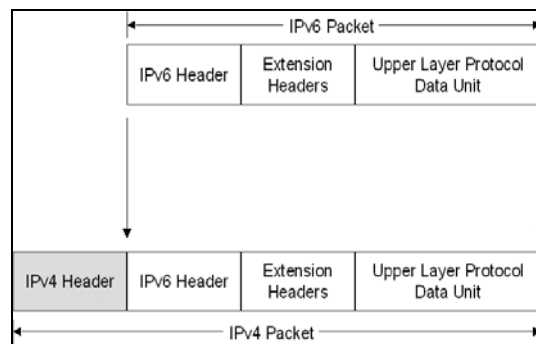
Gambar 5 6 to 4 Tunneling (Rafiudin, 2005)
