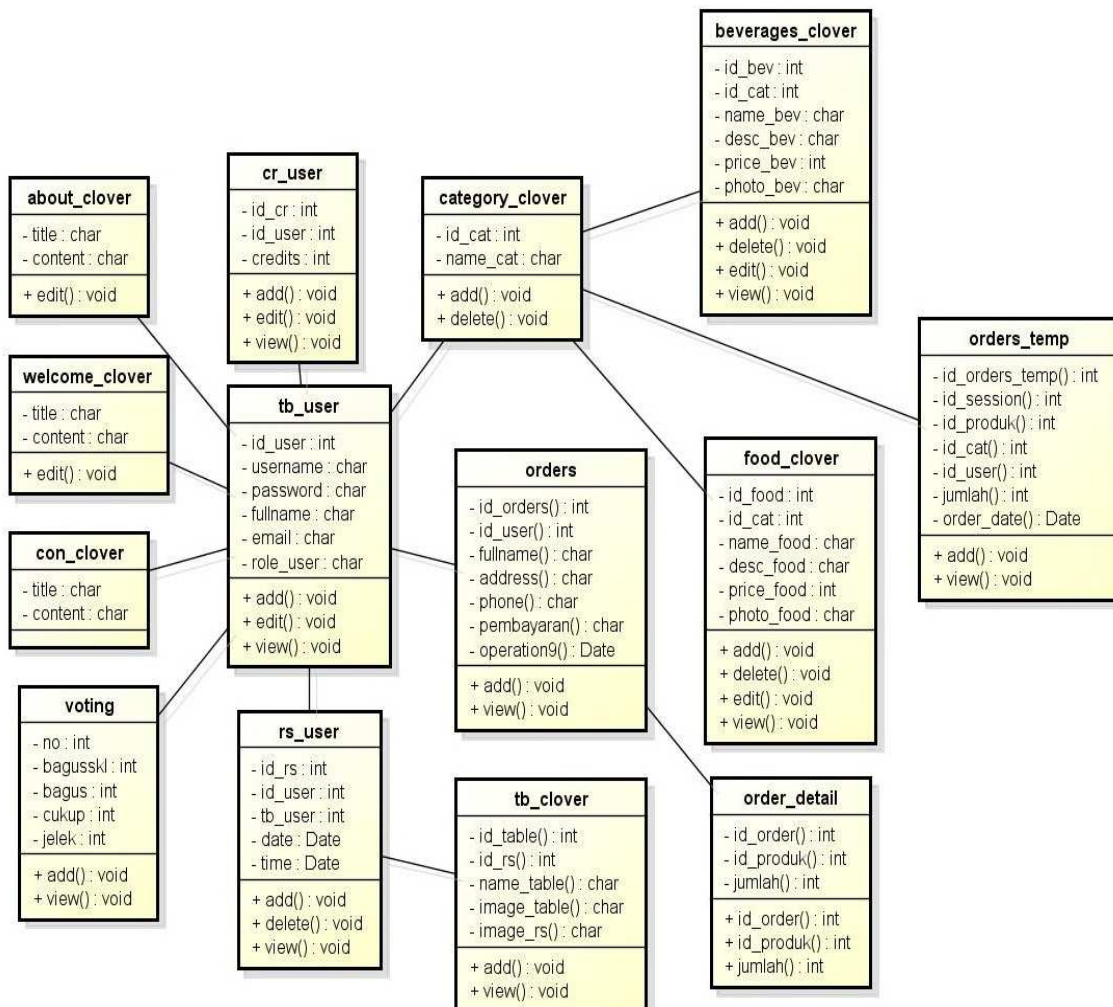
Gambar 9 Class Diagram
