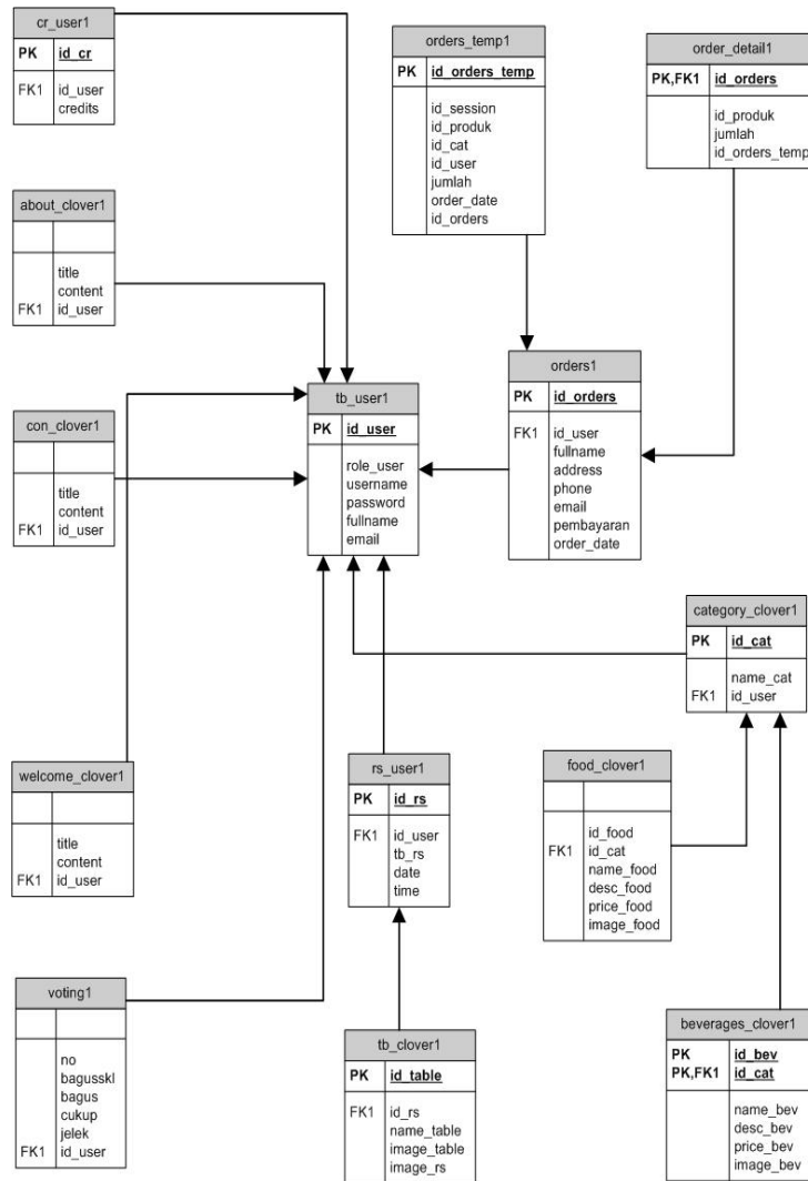
Gambar 11 Diagram Basis Data
