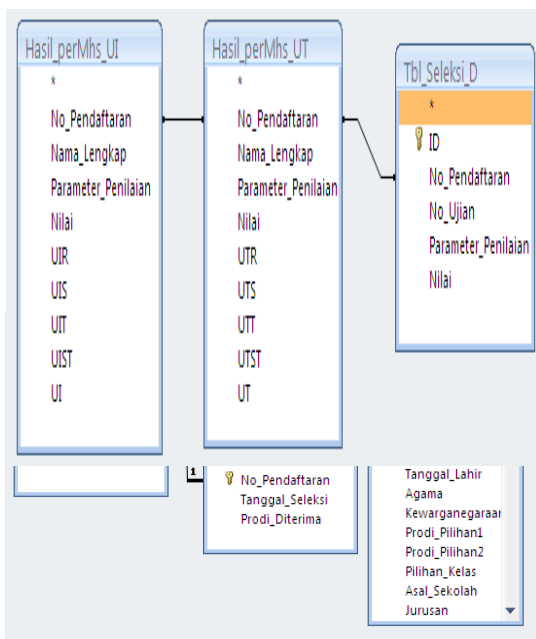
Gambar 3. Diagram E-R
