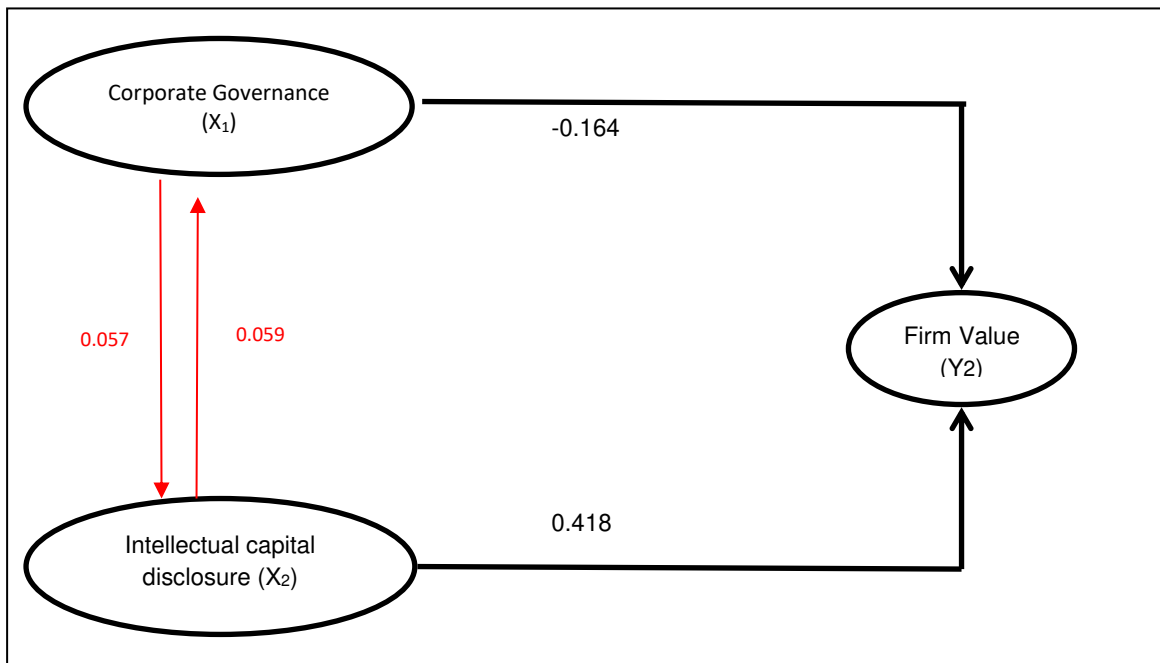
Figure 1. Path Diagram
