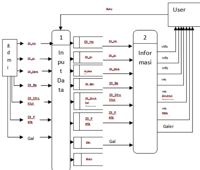
Gambar 2 DFD Level 0
