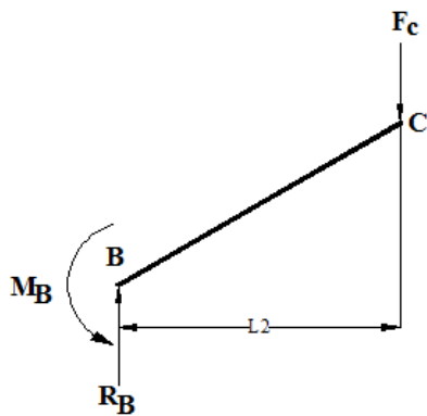
Gambar 4 Diagram benda bebas poros BC
