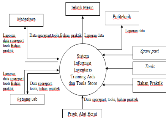
Gambar 1. Gambar Data Flow Diagram
