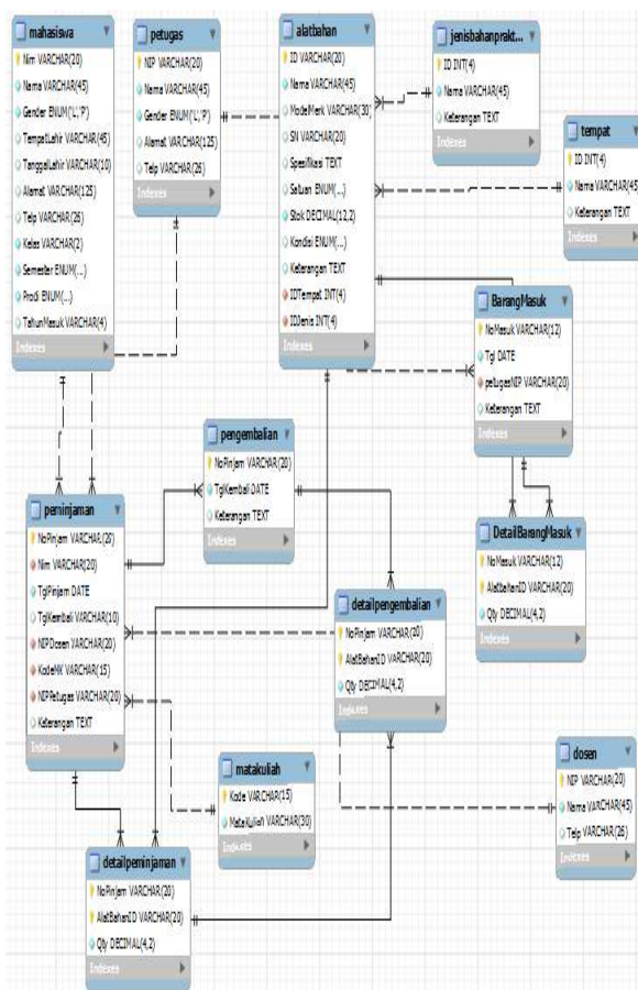
Gambar 2. Enhanced Entity Relationship Diagram
