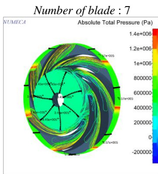
Gambar 7 Inlet-Outlet pressure & Strealine Contour
