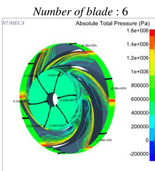
Gambar 6 Inlet-Outlet pressure & Strealine Contour
