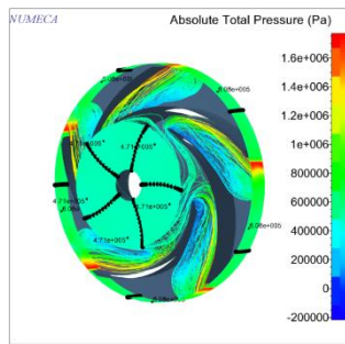
Gambar 5 Inlet-Outlet pressure & Strealine Contour
