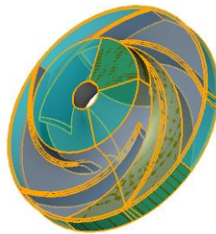
Gambar 3 Finishing Model Impeller
