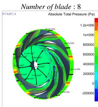
Gambar 8 Inlet-Outlet pressure & Strealine Contour
