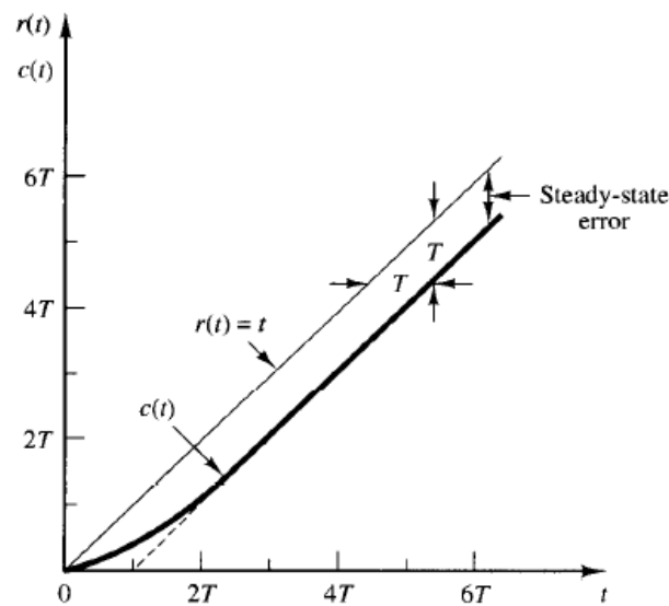
Gambar.6. Steady state ramp error [5]
