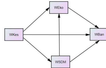
Gambar. 2. Diagram Jalur Model Spasial
