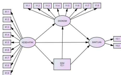
Gambar. 1. Diagram Jalur Model Konseptual
