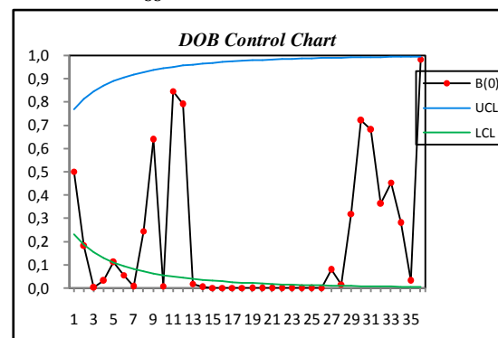
Gambar 2. Diagram Kontrol DOB
